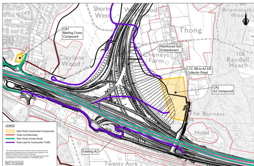
Plate 7.6 Location of reinforced soil embankment
