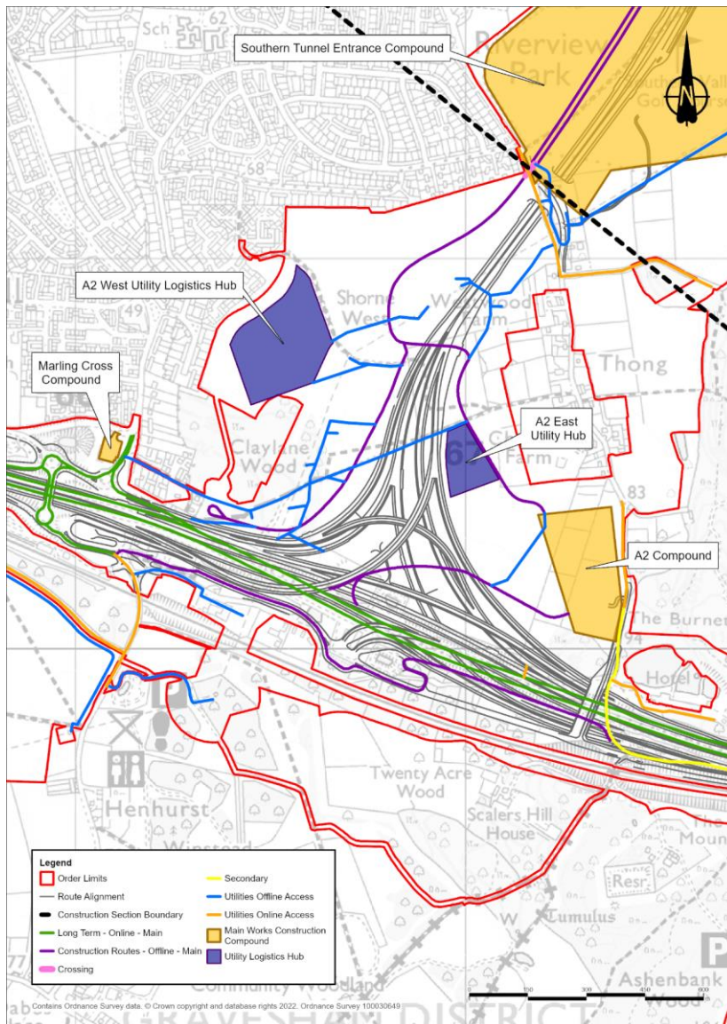
Plate 5.1 Compounds, ULH and construction access routes including utilities (A2 to Thong Lane over the A12)
